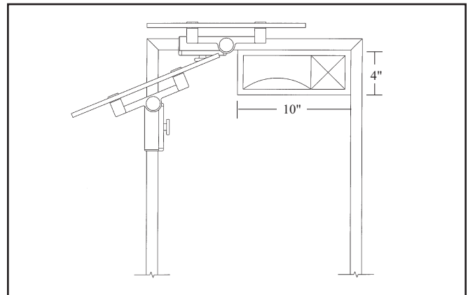
Z9930 with Hatco Heat Lamp and Light
