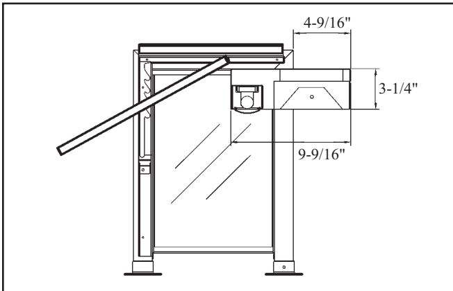
DECO-250 with Hatco Heat Lamp and T8 Lamp
