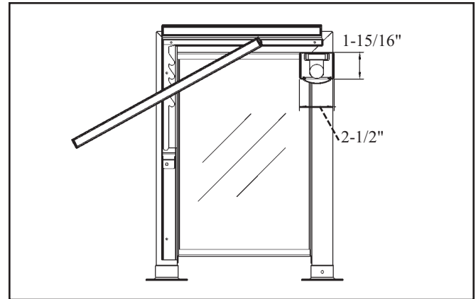
DECO-250 with T8 Light
