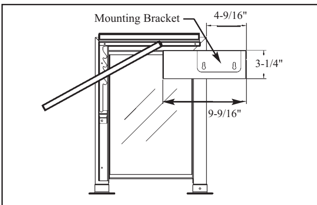
DECO-250 with Shroud and Mounting Bracket
