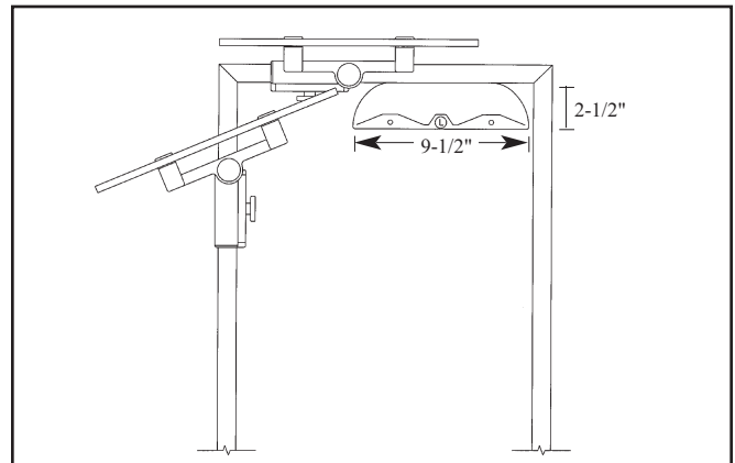
Z9930 with Stealth Double Warmer and Light Combo
