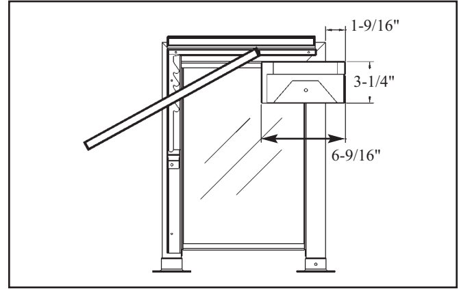
DECO-250 with Hatco Heat Lamp
