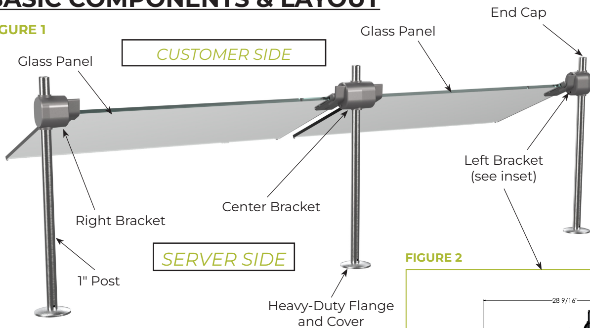
Fig. 1 shows two glass panels with a center bracket.
