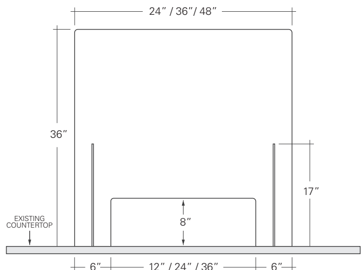
Left: BSI-PWPT (with pass thru) Right: BSI-PW (without pass thru)
